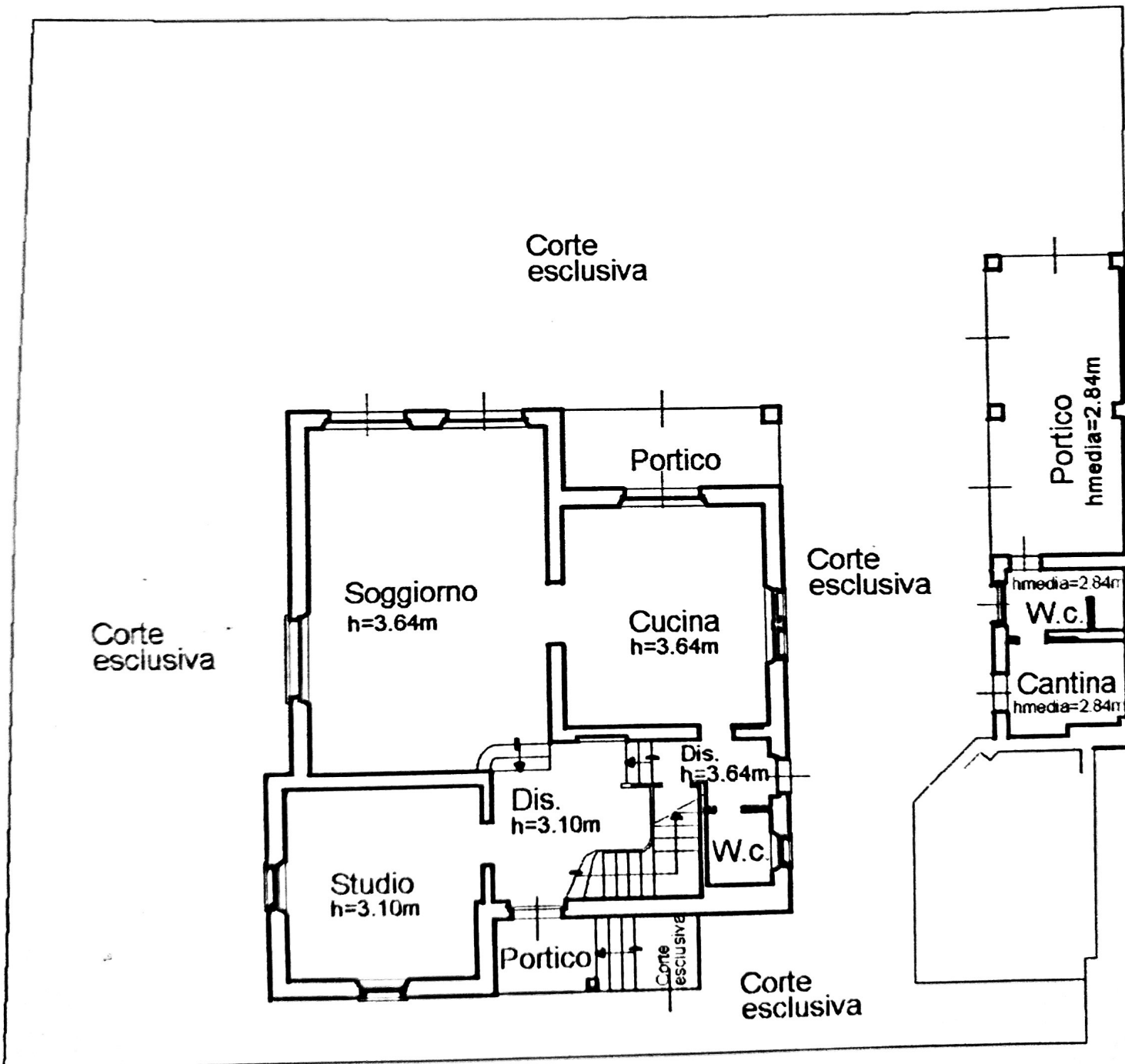
PIANO TERRA
